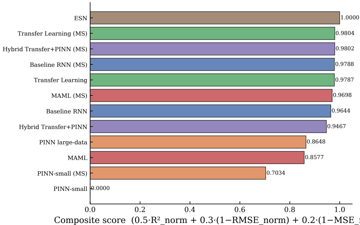
MG — Composite Score Leaderboard
